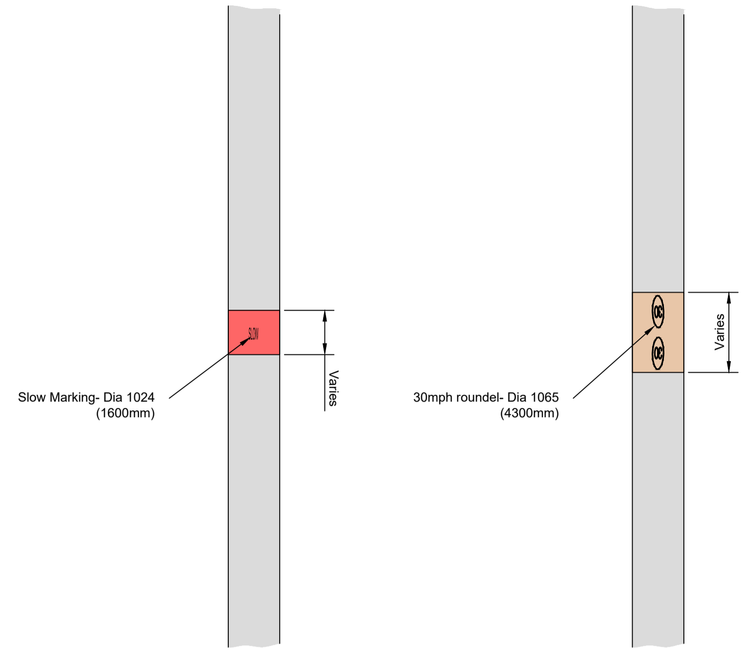
Typical 'SLOW' markings (1600mm) on 'red' Clause 924 background Detail A Scale 1:500
